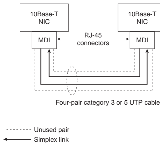
Figure 7-15 The Typical 10Base-T Link Is a Four-Pair UTP Cable in Which Two Pairs Are Not Used
