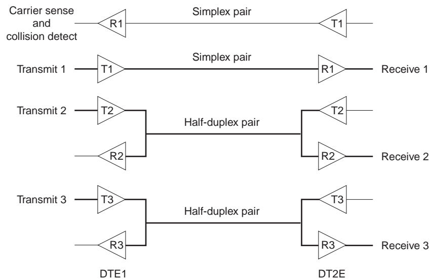
Figure 7-18 The 100Base-T4 Wire-Pair Usage During Frame Transmission
