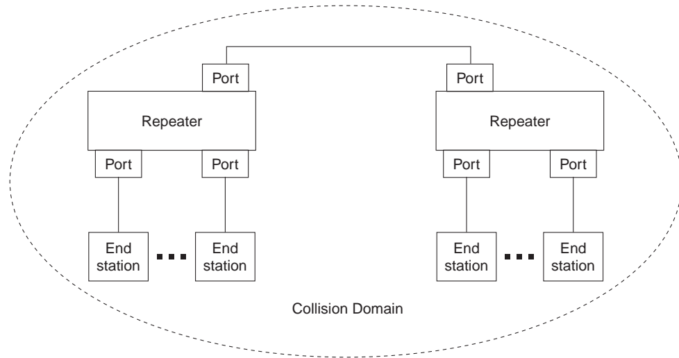
(a) Repeater-based CSMA/CD network
