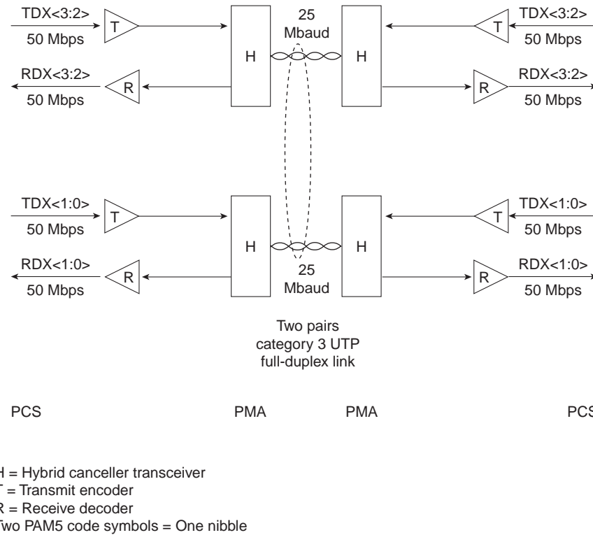
Figure 7-20 The 100Base-T2 Link Topology
