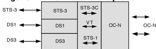
Figure 20. Terminal Multiplexer
