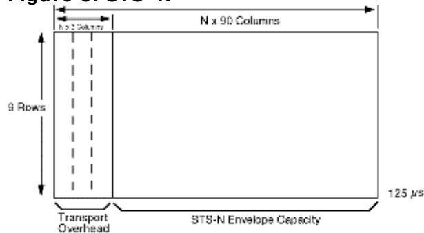
Figure 5. STS-N
