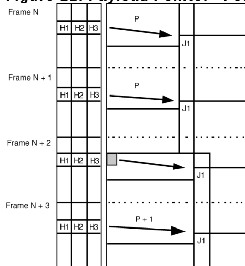
Figure 12. Payload Pointer—Positive Justification
