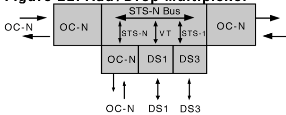
Figure 22. Add/Drop Multiplexer
