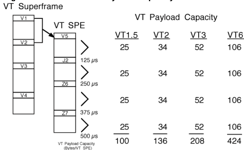
Figure 18. VT SPE and Payload Capacity
