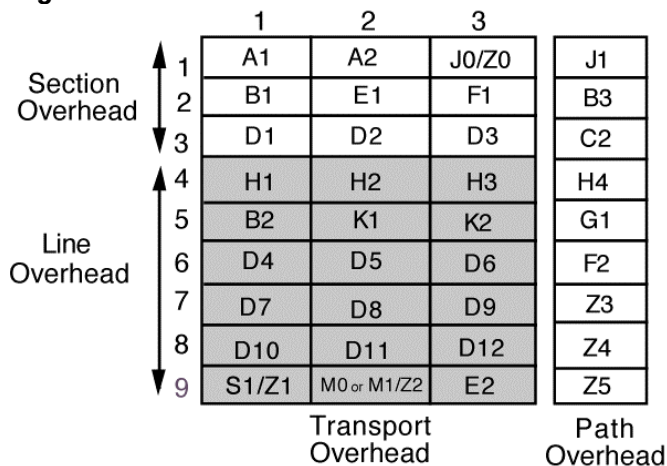
Figure 8. Line Overhead: Rows 4 to 9 of Transport Overhead
