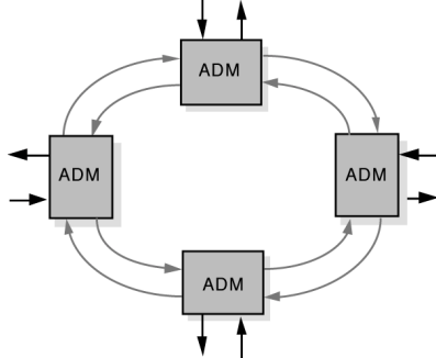
Figure 29. Ring Architecture
