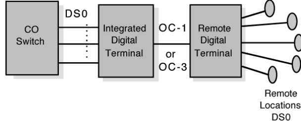
Figure 25. Integrated Digital Loop Carrier
