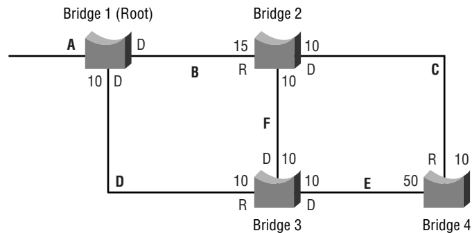
FIGURE 14.9 Path selection in a bridged environment
