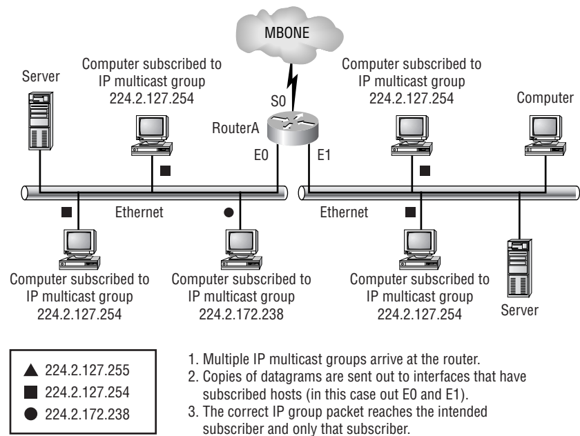
FIGURE 12.3 Multicast communication
