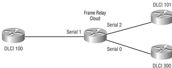
FIGURE 5.16 A Physical Frame Relay Network
