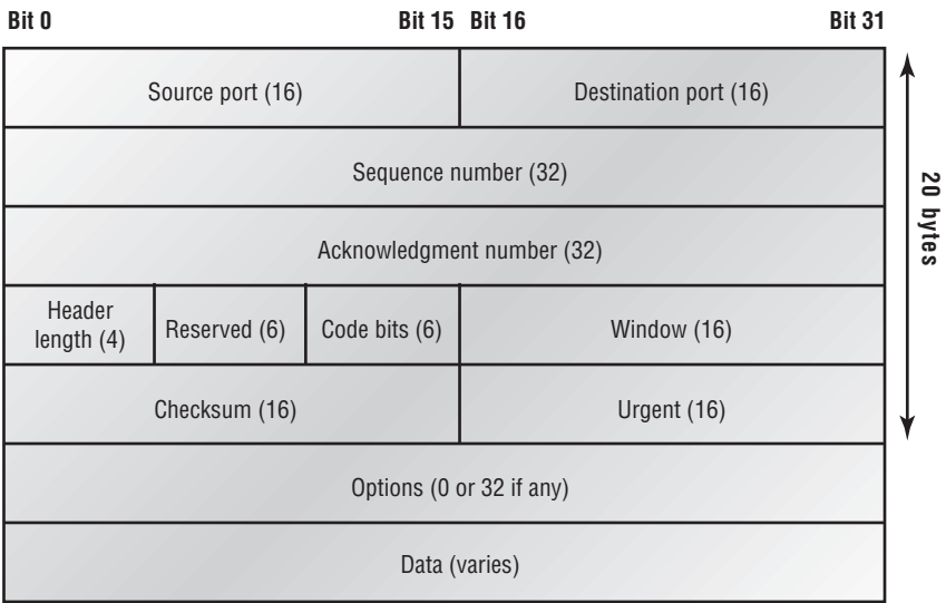
FIGURE 7.3 TCP segment format
