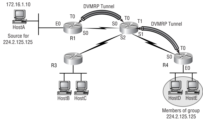
FIGURE 12.16 DVMRP tunnels
