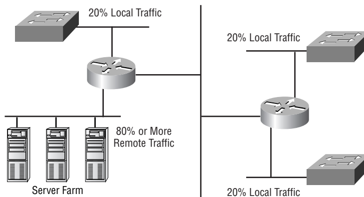
FIGURE 19.2 The 20/80 Network
