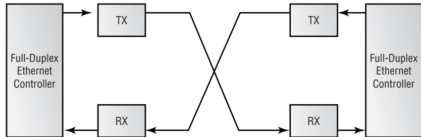
FIGURE 2.5 Full-duplex circuitry
