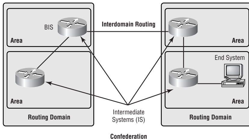
FIGURE 8.11 IS-IS terminology
