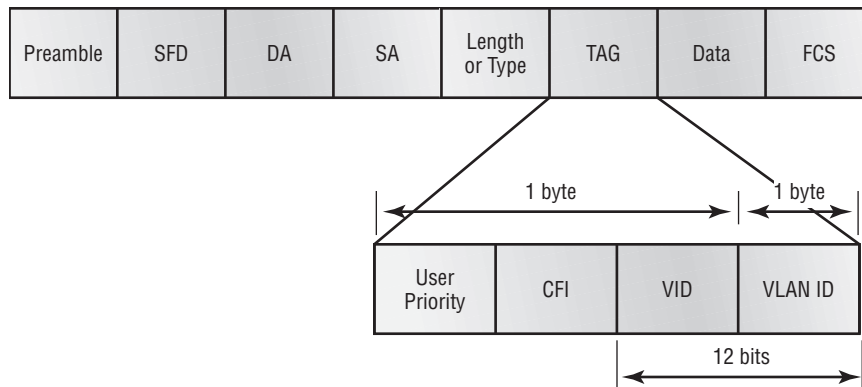
FIGURE 2.4 The VLAN tag frame format
