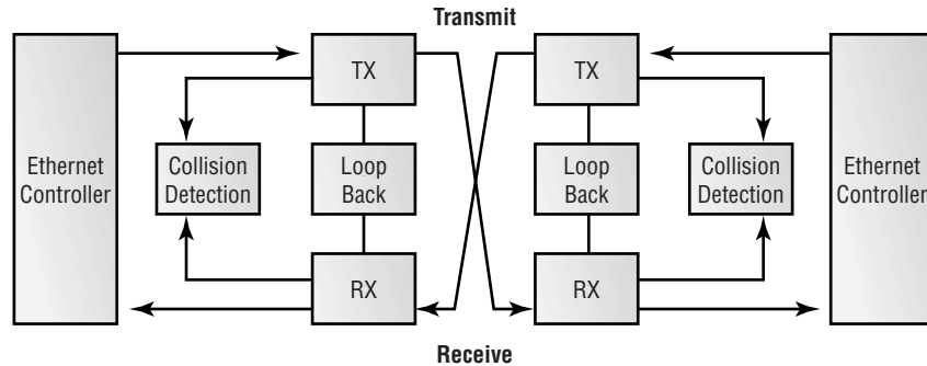
FIGURE 2.6 Half-duplex circuitry
