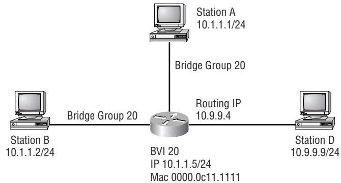
FIGURE 14.12 Integrated routing and bridging
