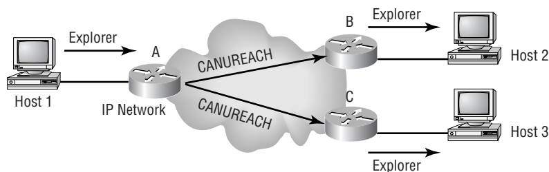
FIGURE 15.3 DLSw explorers and CANUREACH frames
