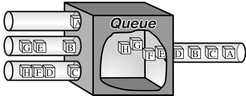
FIGURE 13.6 Priority assignment using Weighted Fair Queuing
