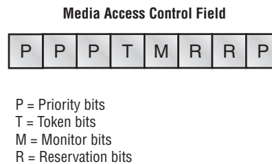
FIGURE 2.9 Token Ring media access control field
