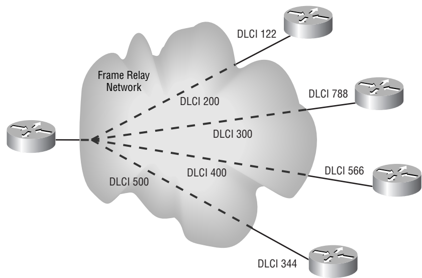
FIGURE 5.5 A Star Topology with DLCIs
