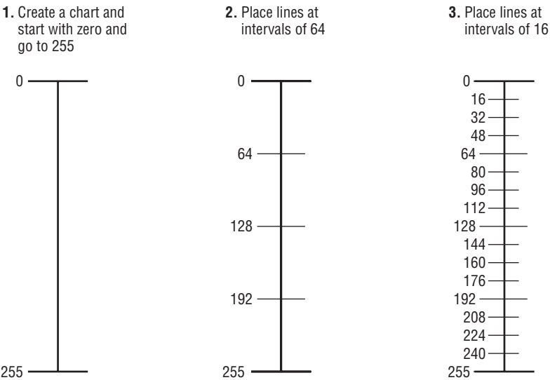
FIGURE 7.13 The three steps in creating a VLSM table
