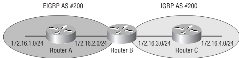
FIGURE 10.8 EIGRP and IGRP interaction
