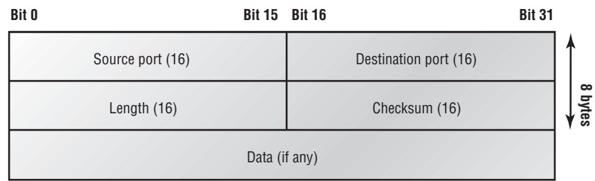
FIGURE 7.4 UDP segment
