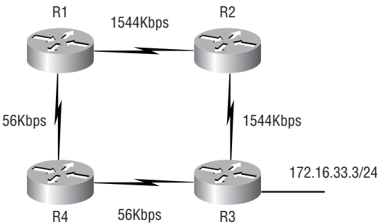
FIGURE 8.5 Bandwidth and path selection
