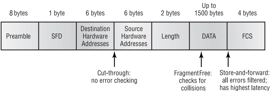
FIGURE 19.9 Different switching modes within a frame
