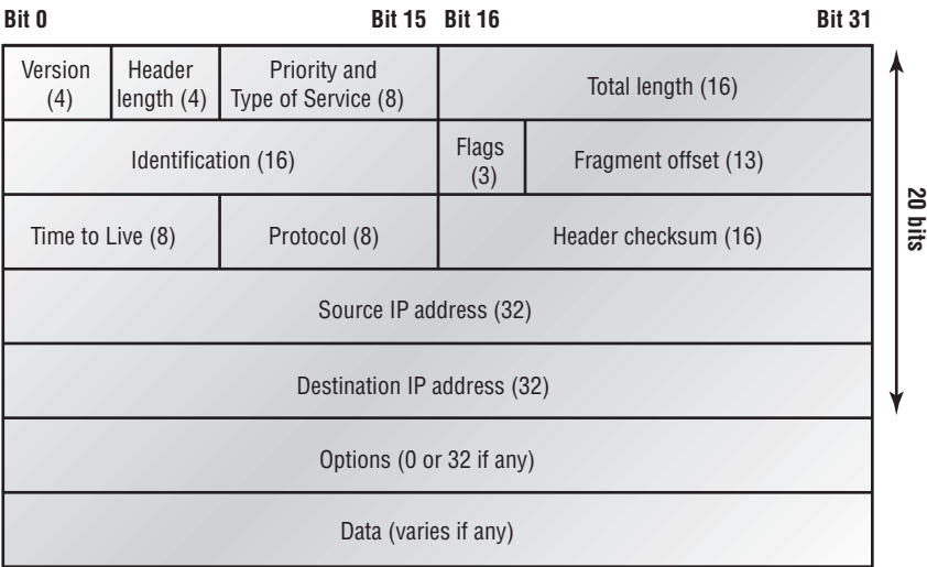
FIGURE 7.6 IP Header
