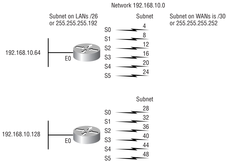
FIGURE 7.12 14 subnets with VLSM applied
